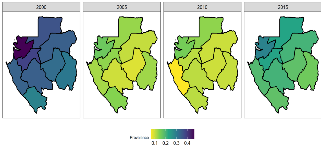
Fig. 3 Map of malaria prevalence in Gabon by year (2000, 2005, 2010, 2015). This plot presents the estimate obtained with the smoothing model and survey complexity
