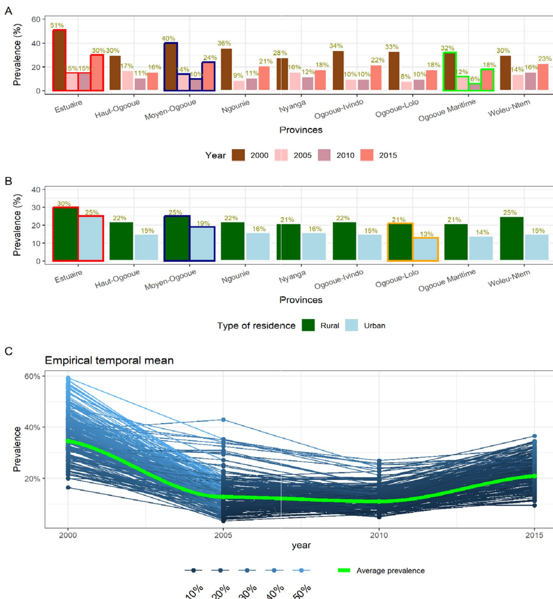
Fig. 2 An overview of the distribution of the prevalence. A the variation of the prevalence over time by province. The colors red and blue highlight the first two provinces with high prevalence. The green color highlights the province where the prevalence reached the lowest value. B distribution of the prevalence by type of residence for each province. C prevalence for each cluster over time with the green line showing the overall trend based on polynomial functions
