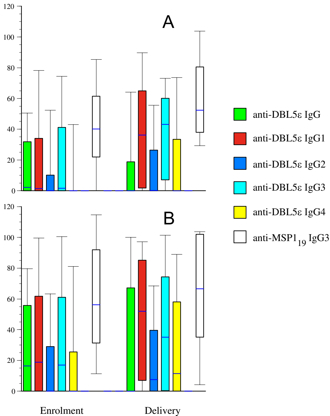
Figure 1 Parity-dependency of the plasma antibody reactivity to VAR2CSA and MSP1 19 recombinant proteins. ELISA was carried out on DBL5ε- and MSP1 19 coated plates. IgG, IgG1, IgG2, IgG3, and IgG4 directed against DBL5ε-, as well as against MSP1 19 . Antibody plasma levels are expressed as arbitrary units (AU) and are shown at enrolment and at delivery for primigravids (panel A, n = 53) and multigravids women (panel B, n = 185) from Senegal. The top, bottom, and line through the middle of the box correspond to the 75 th percentile, 25 th percentile, and 50 th percentile (median), respectively. The whiskers on the bottom extend from the 10 th percentile and top 90 th percentile.
