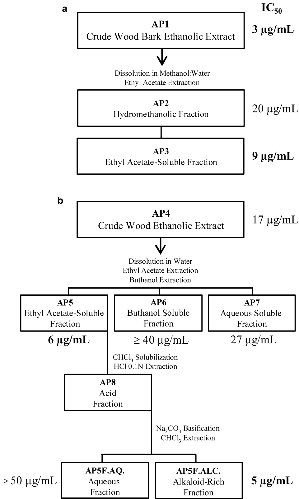
Fig. 2 Fractionation workflow of the plant stem bark (a), and stem (b) extracts from Aspidosperma pyrifolium . The in vitro activity against P. falciparum (IC 50 ) highlighted in bold represents the best results
