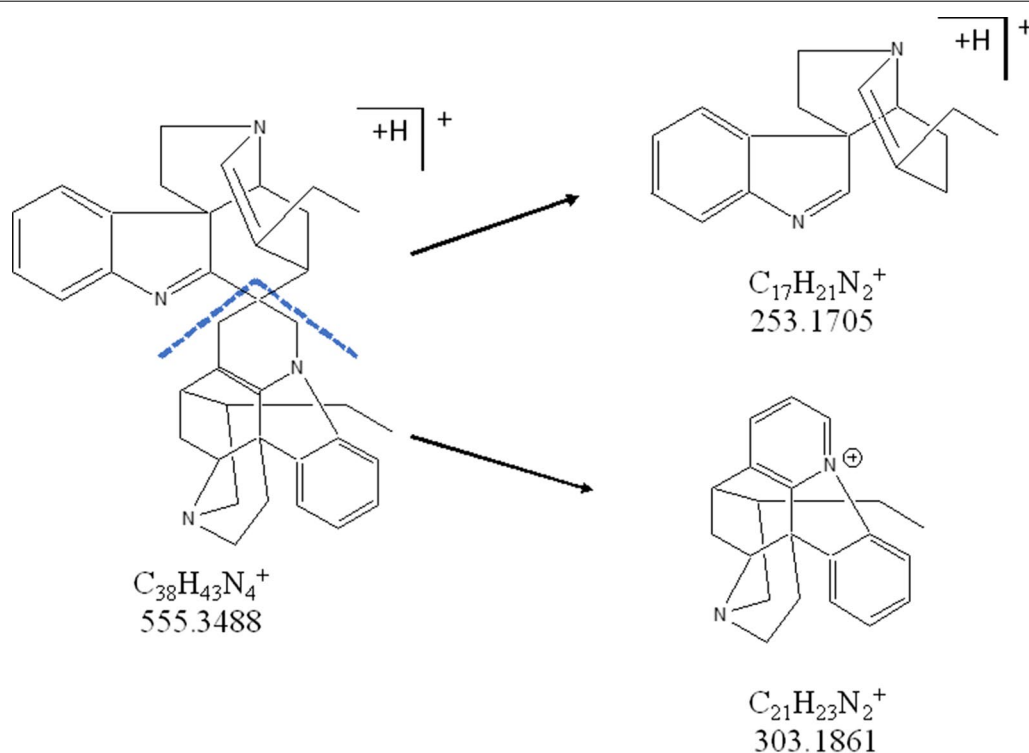
Fig. 4 Putative fragmentation of compound A (Leucoridine B)
